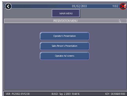
Figure 16 - Presentation Menu
